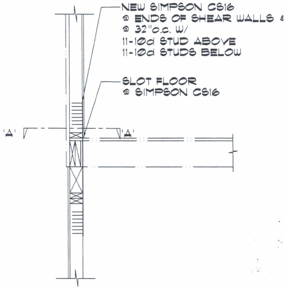
SECT. 'A-A'
