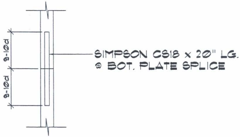
SECT. 'A-A'
