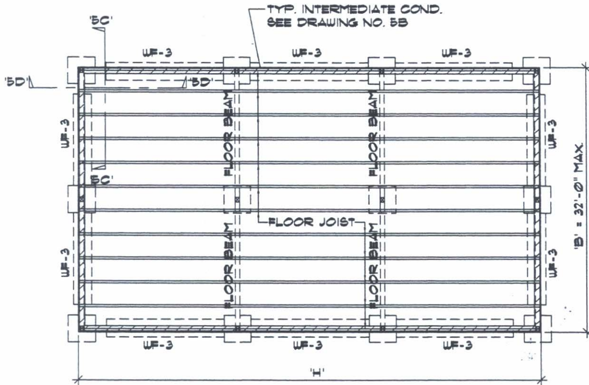
EXISTING CONDITION
