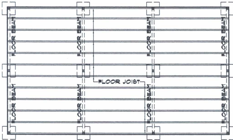
EXISTING CONDITION
