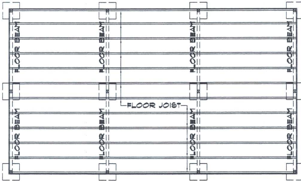
EXISTING CONDITION
